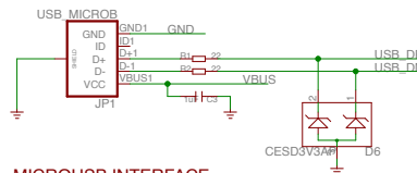
MICROUSB INTERFACE
