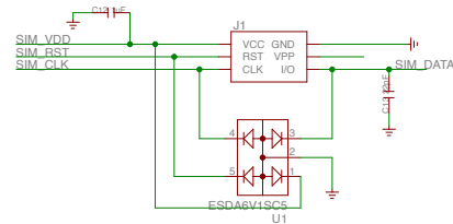
SIMCARD HOLDER
